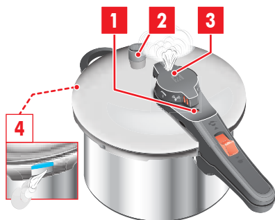
Abb. 1: Safety functions
